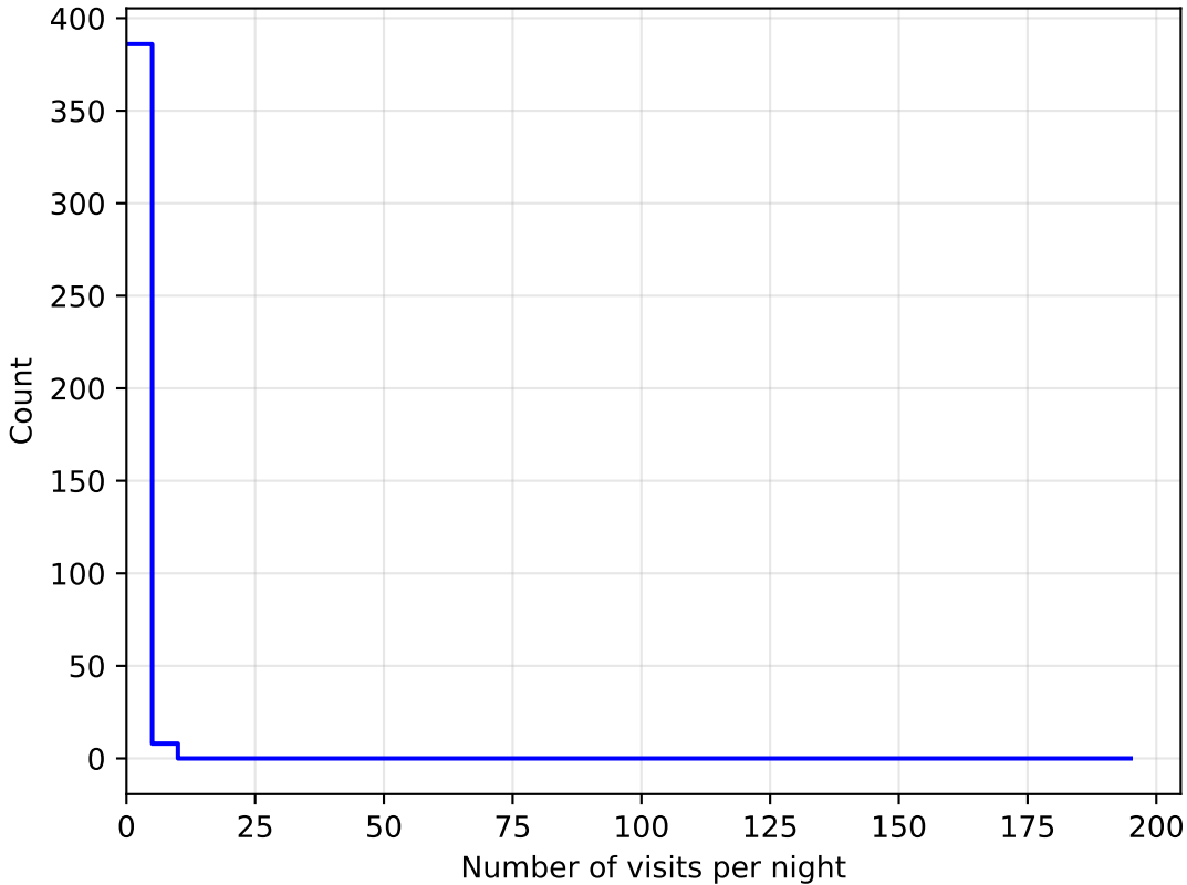
weather_cloudso18v3.4_10yrs all bands: DD:WFD NVisitsPerNight
