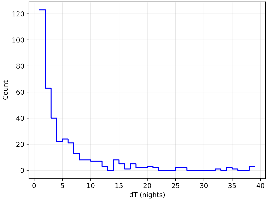
weather_cloudso18v3.4_10yrs all bands: DD:WFD Delta Nights Histogram
