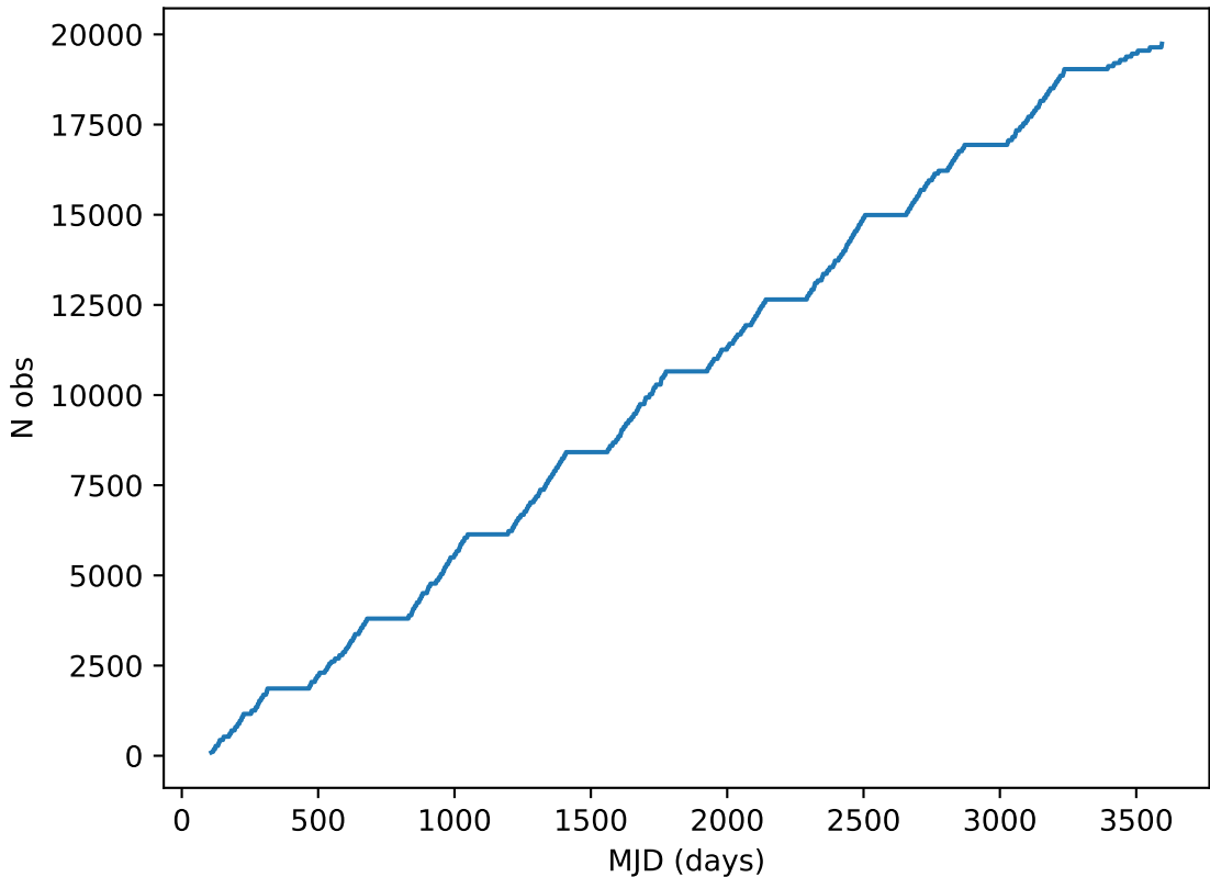
weather_cloudso18v3.4_10yrs all bands: DD:EDFS Cumulative NVisits
