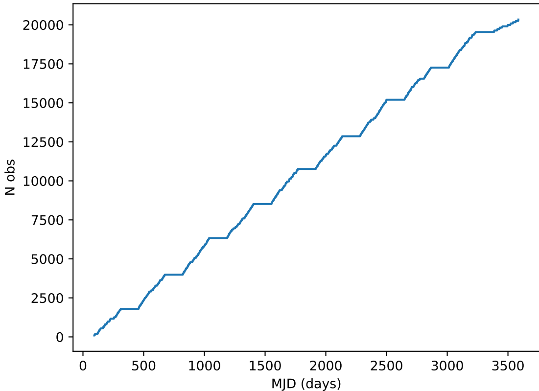
weather_cloudso18v3.4_10yrs all bands: DD:ECDFS Cumulative NVisits
