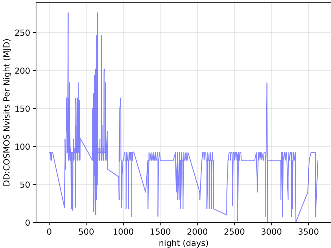
weather_cloudso18v3.4_10yrs all bands: DD: COSMOS Nvisits Per Night
