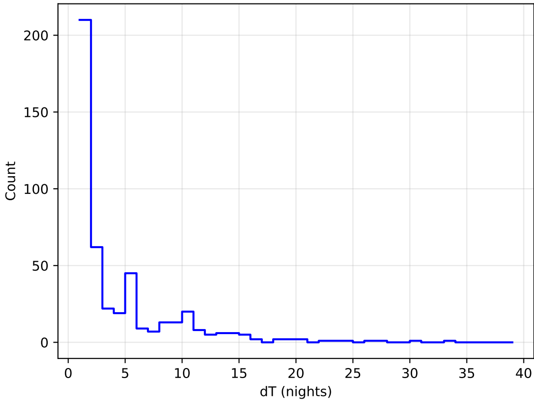
weather_cloudso18v3.4_10yrs all bands: DD: COSMOS Delta Nights Histogram
