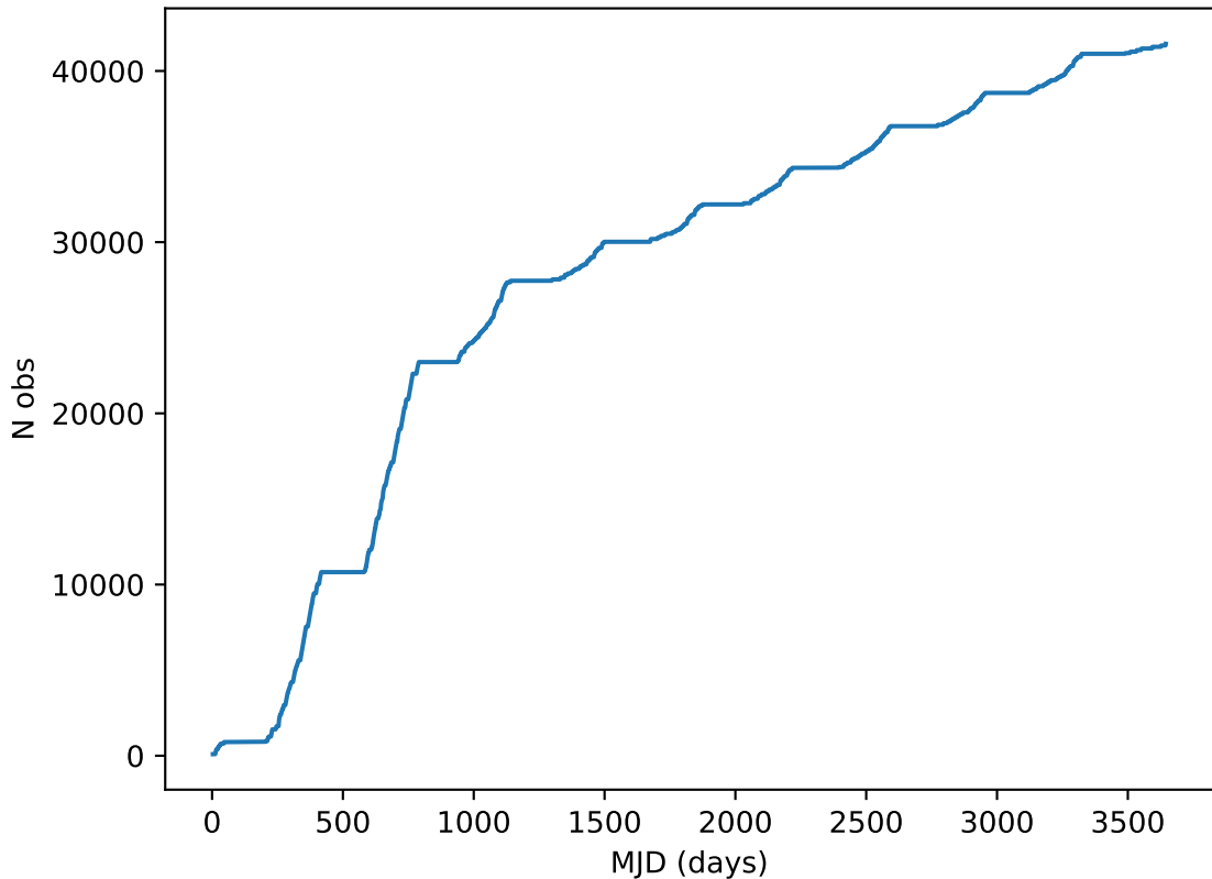
weather_cloudso18v3.4_10yrs all bands: DD:COSMOS Cumulative NVisits
