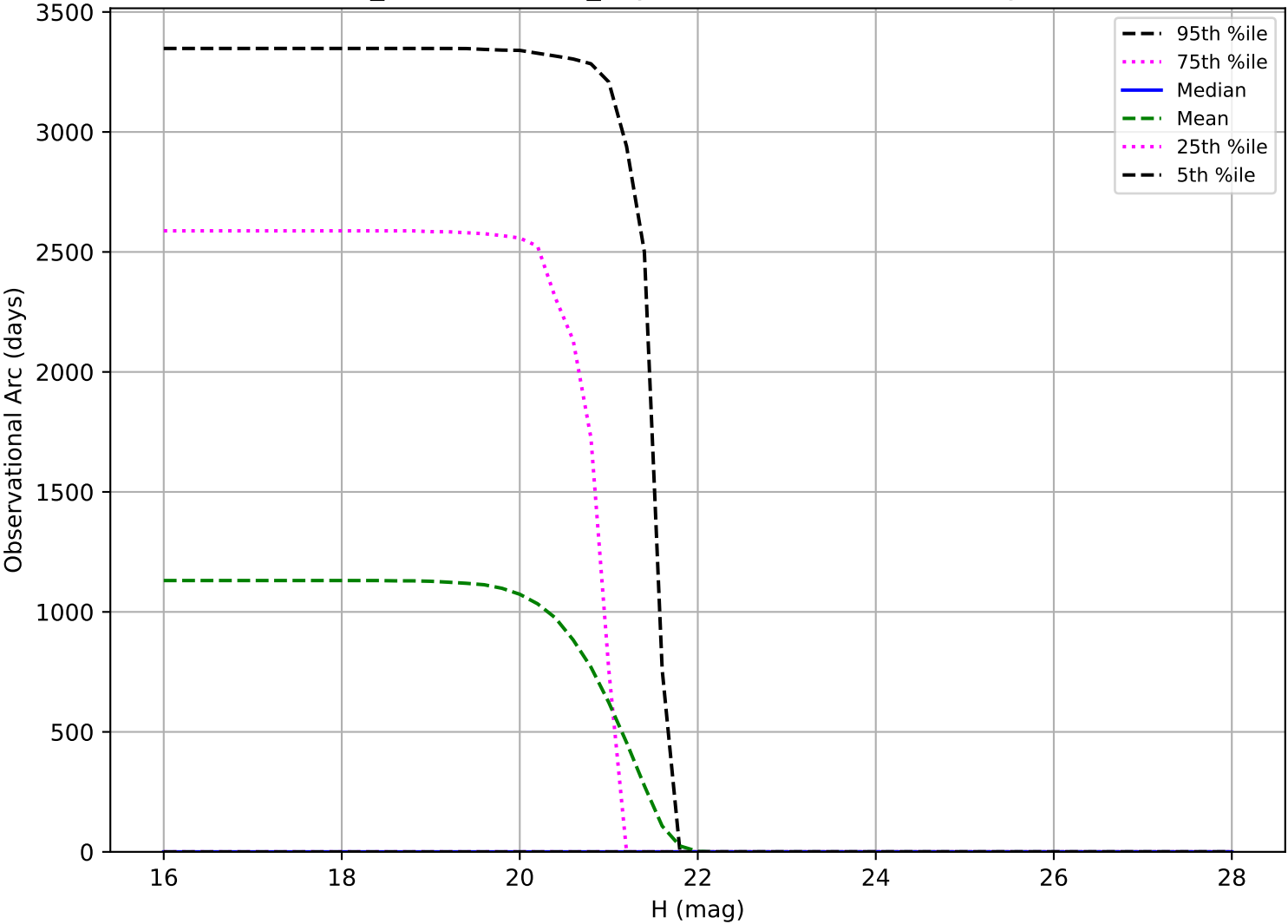
weather_cloudso16v3.4_10yrs: Observational Arc Length Vatra
