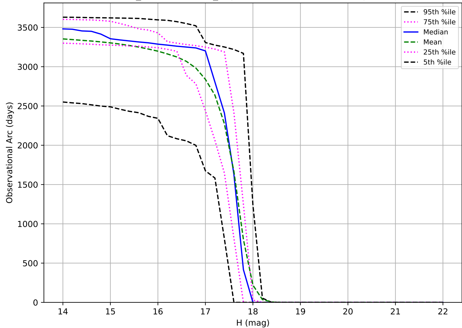
weather_cloudso16v3.4_10yrs: Observational Arc Length Trojan
