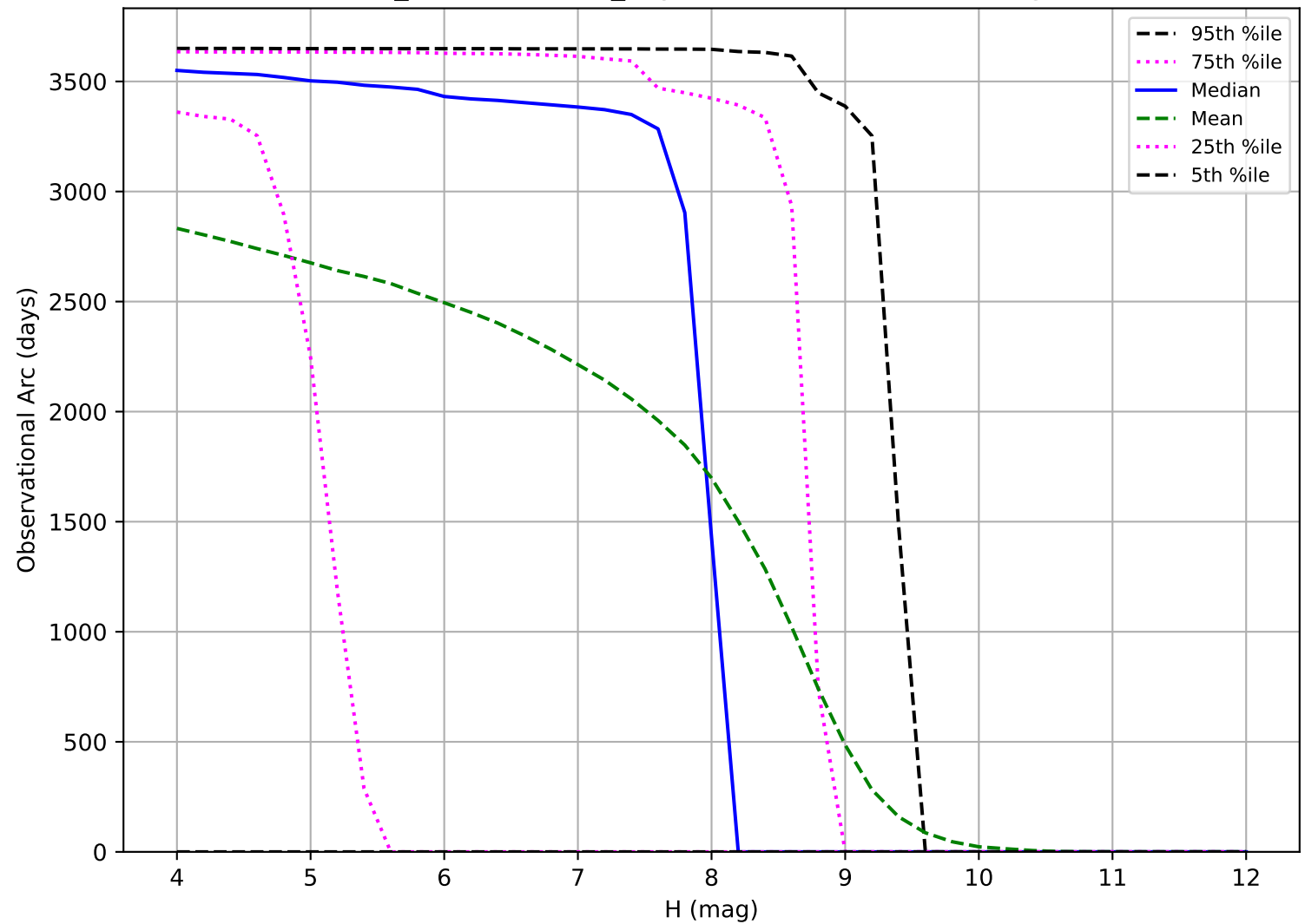
weather_cloudso16v3.4_10yrs: Observational Arc Length TNO
