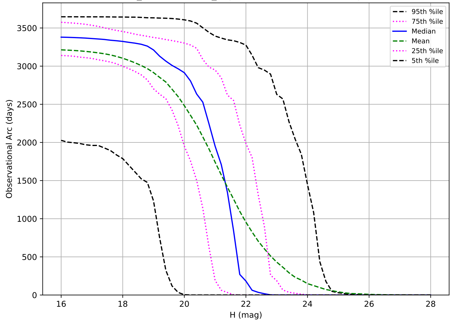
weather_cloudso16v3.4_10yrs: Observational Arc Length PHA
