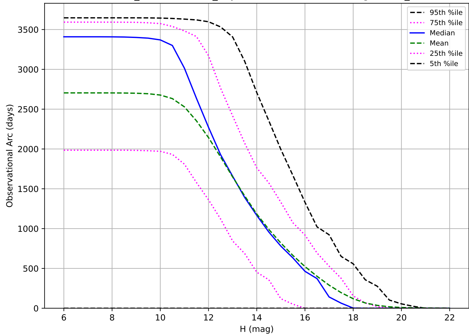
weather_cloudso16v3.4_10yrs: Observational Arc Length OCC_r5
