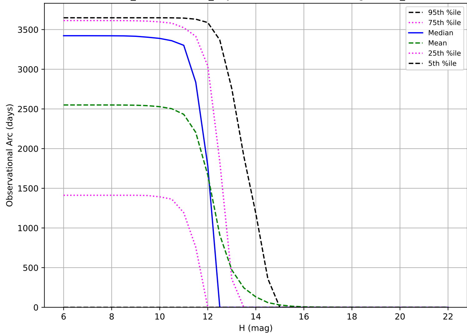
weather_cloudso16v3.4_10yrs: Observational Arc Length OCC_r20
