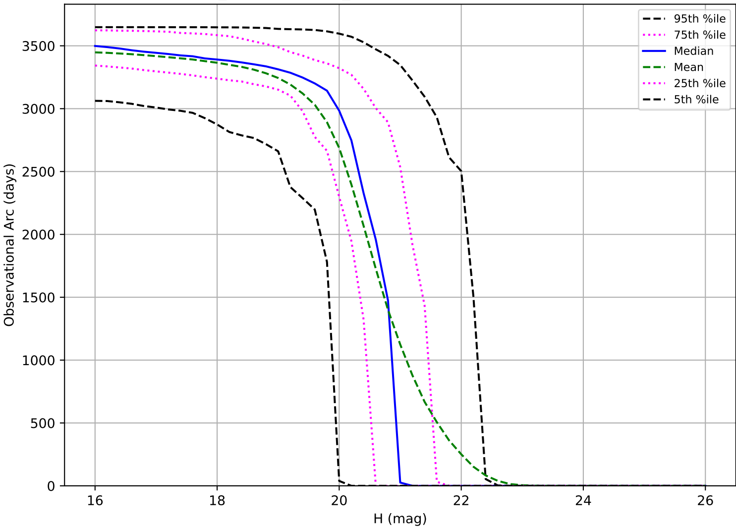
weather_cloudso16v3.4_10yrs: Observational Arc Length MBA
