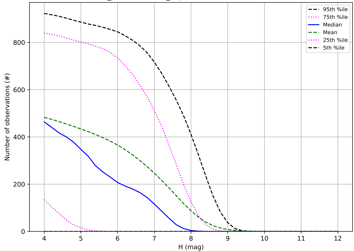
weather_cloudso16v3.4_10yrs: Number of observations TNO
