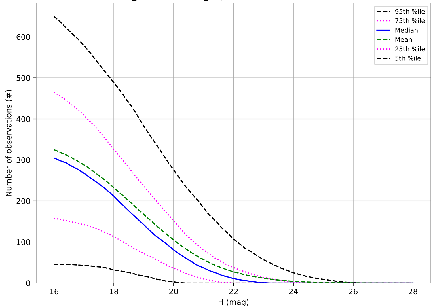
weather_cloudso16v3.4_10yrs: Number of observations PHA
