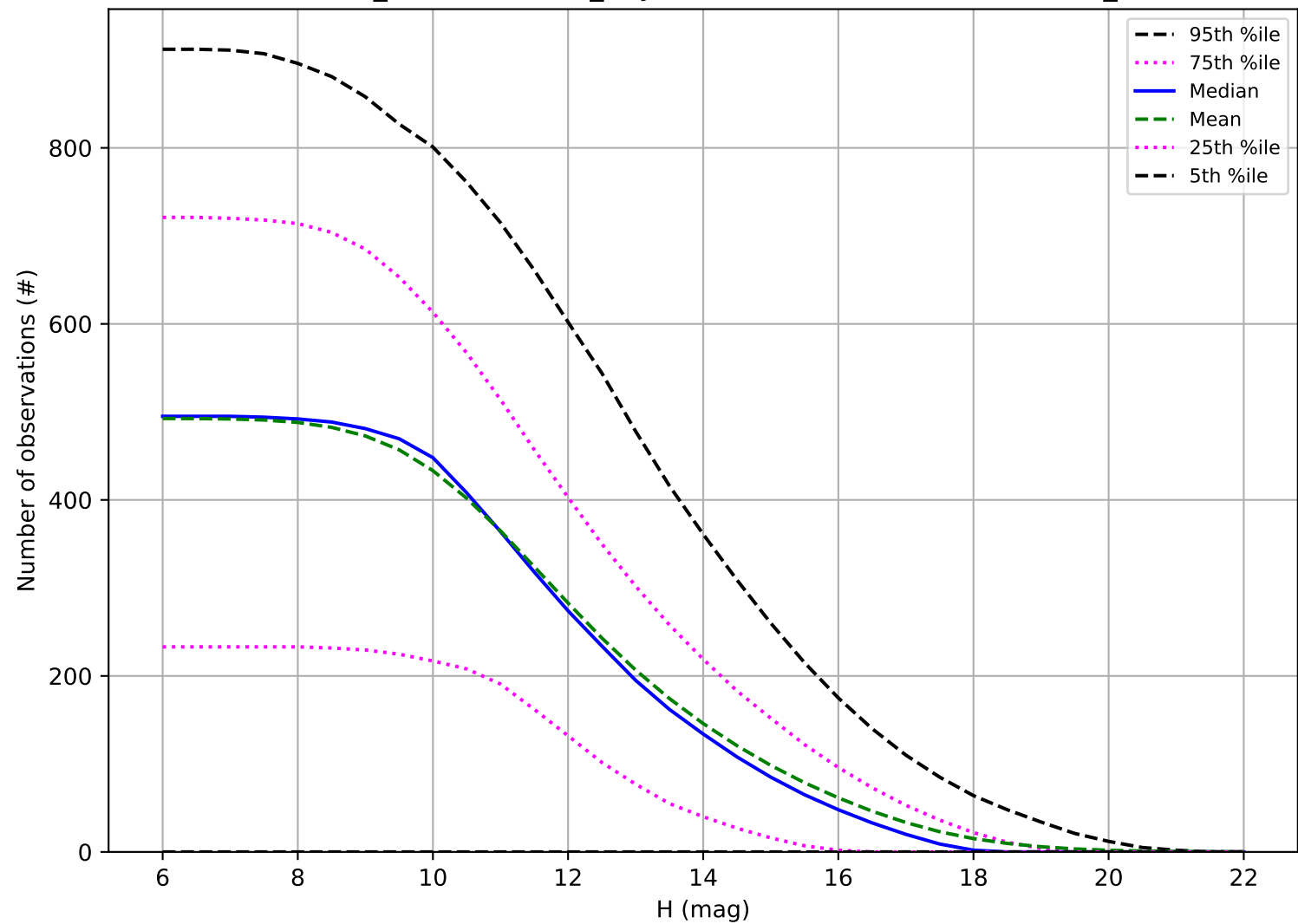
weather_cloudso16v3.4_10yrs: Number of observations OCC_r5
