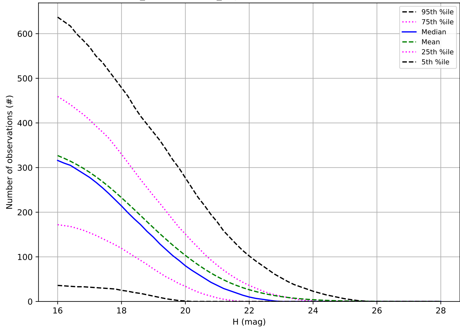
weather_cloudso16v3.4_10yrs: Number of observations NEO
