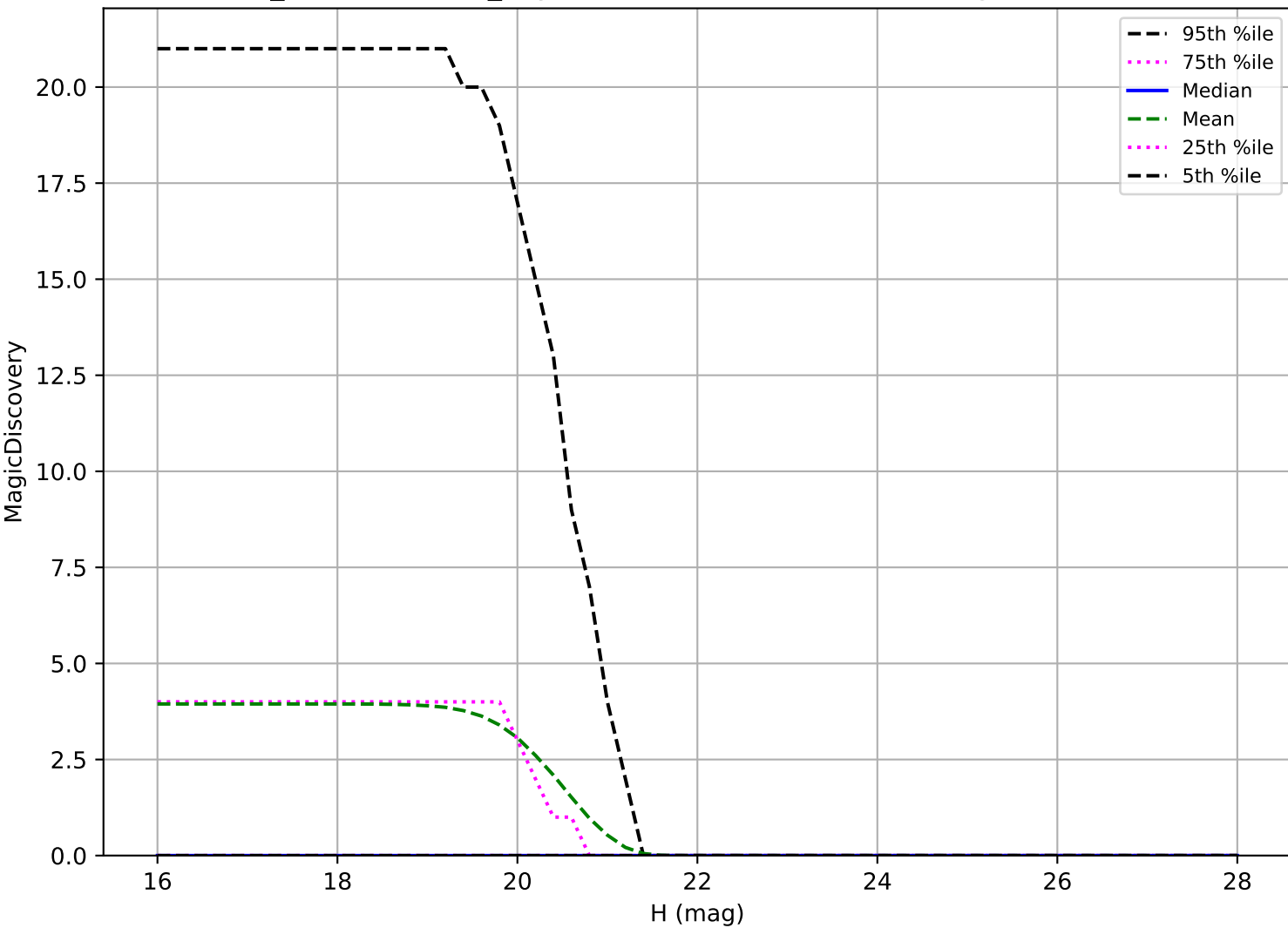
weather_cloudso16v3.4_10yrs: Vatira 6 detections in 60 nights detection loss
