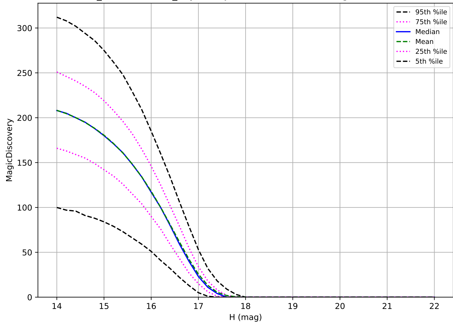
weather_cloudso16v3.4_10yrs: Trojan 6 detections in 60 nights detection loss
