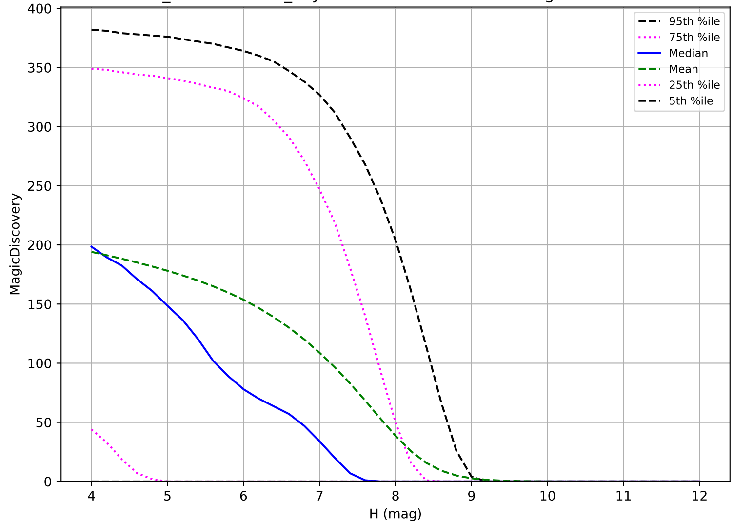
weather_cloudso16v3.4_10yrs: TNO 6 detections in 60 nights detection loss
