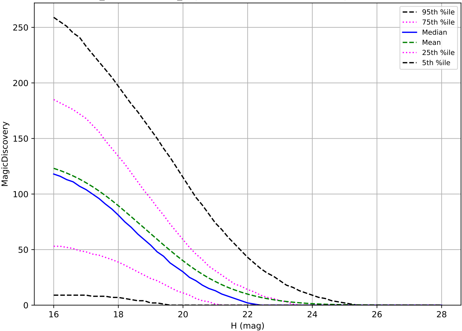
weather_cloudso16v3.4_10yrs: PHA 6 detections in 60 nights detection loss
