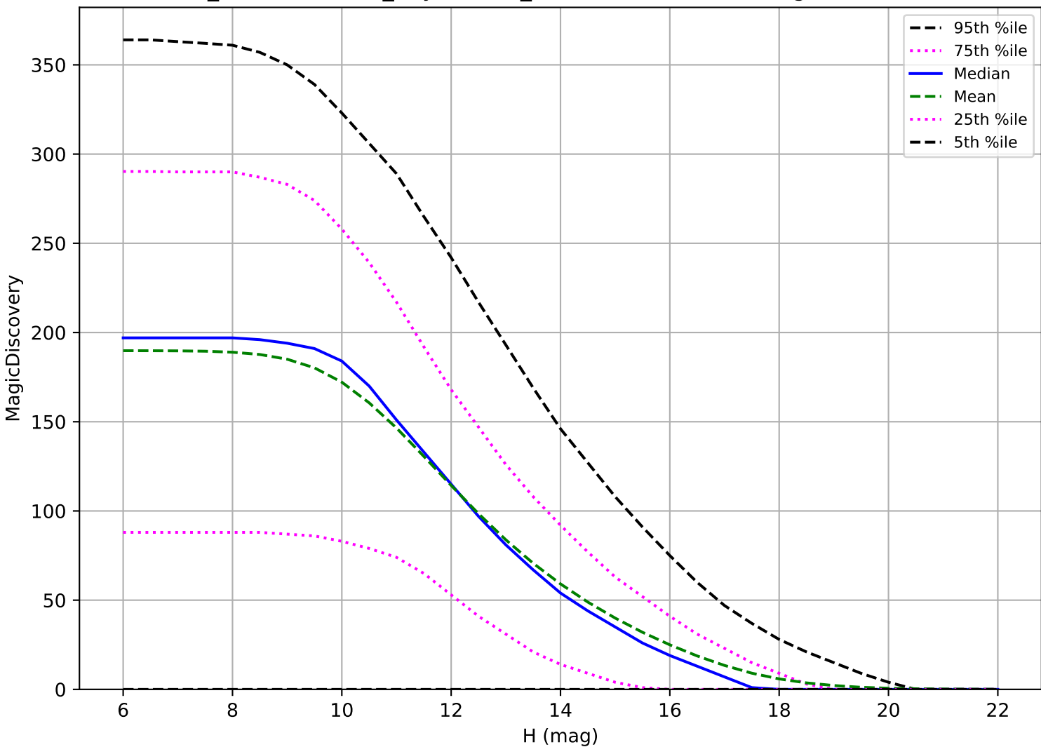
weather_cloudso16v3.4_10yrs: OCC_r5 6 detections in 60 nights detection loss
