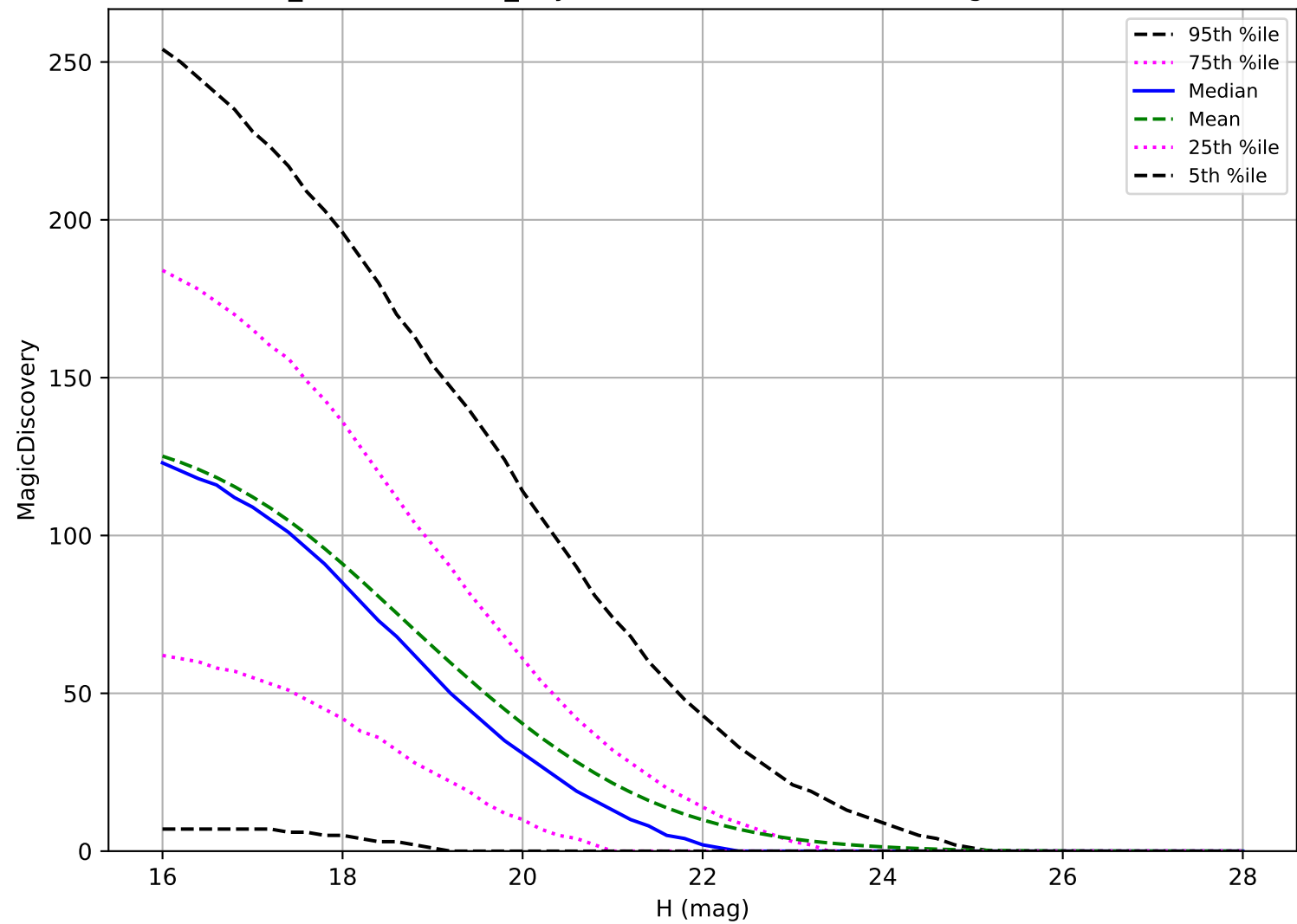
weather_cloudso16v3.4_10yrs: NEO 6 detections in 60 nights detection loss
