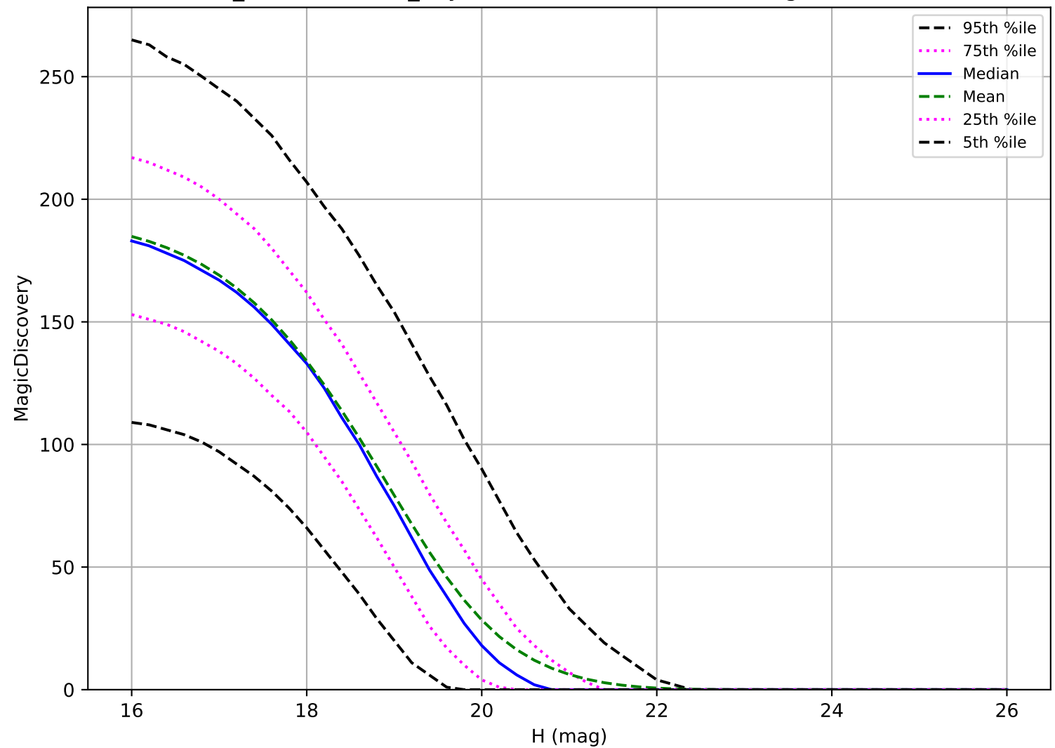
weather_cloudso16v3.4_10yrs: MBA 6 detections in 60 nights detection loss
