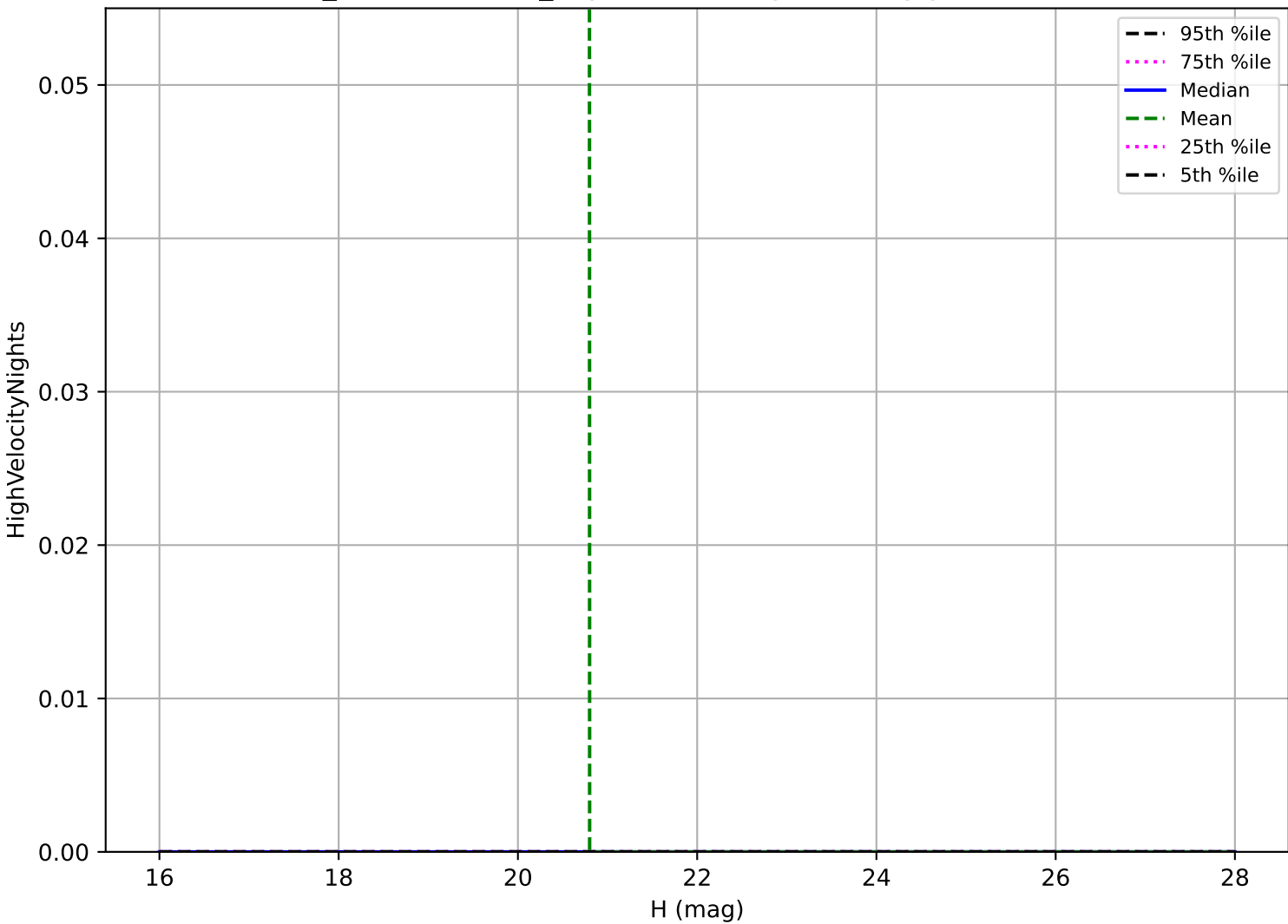
weather_cloudso16v3.4_10yrs: Vatira High velocity pair detection loss
