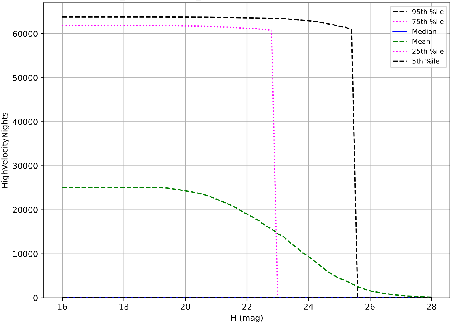
weather_cloudso16v3.4_10yrs: PHA High velocity pair detection loss
