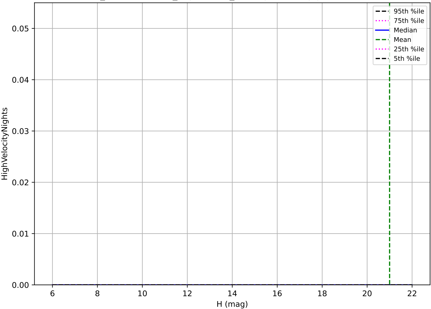
weather_cloudso16v3.4_10yrs: OCC_r20 High velocity pair detection loss
