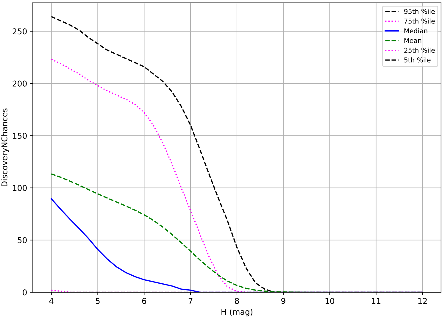
weather_cloudso16v3.4_10yrs: TNO 3 pairs in 15 nights detection loss
