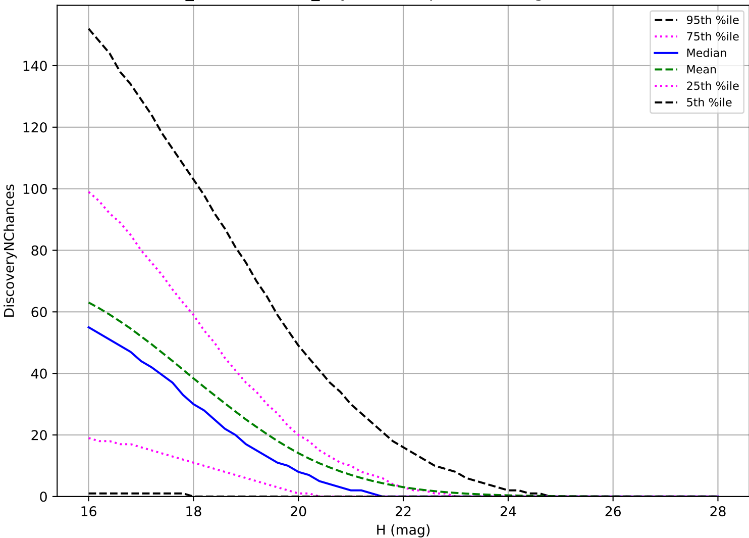
weather_cloudso16v3.4_10yrs: PHA 3 pairs in 15 nights detection loss
