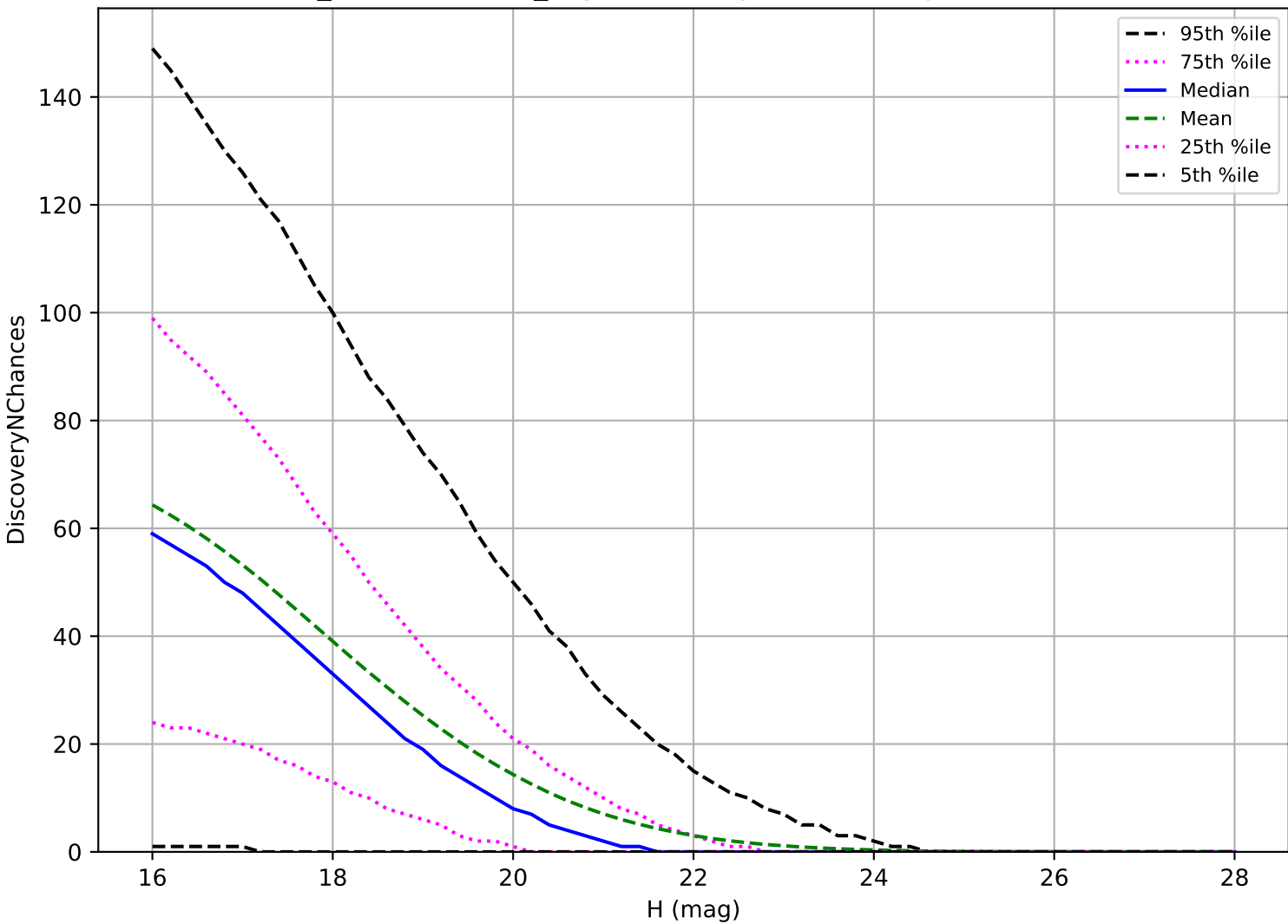
weather_cloudso16v3.4_10yrs: NEO 3 pairs in 15 nights detection loss
