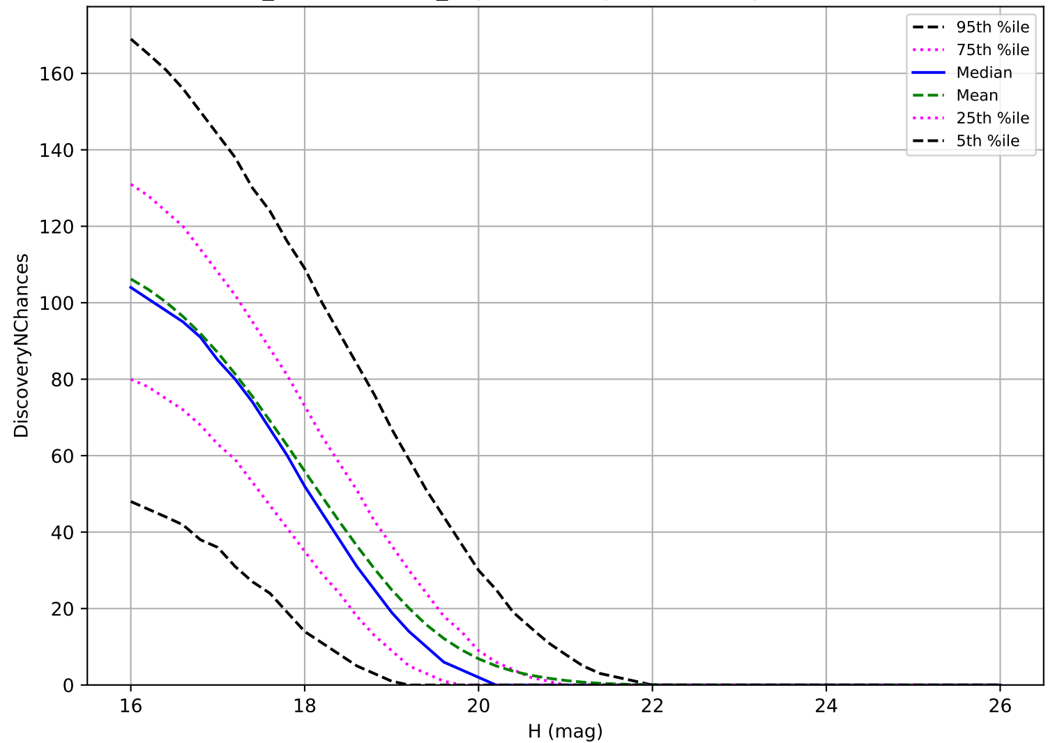
weather_cloudso16v3.4_10yrs: MBA 3 pairs in 15 nights detection loss
