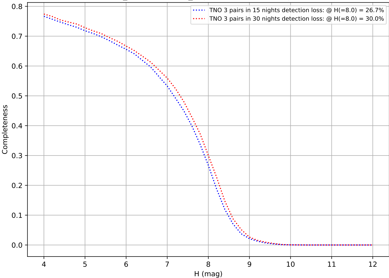
weather_cloudso16v3.4_10yrs: DifferentialCompleteness
