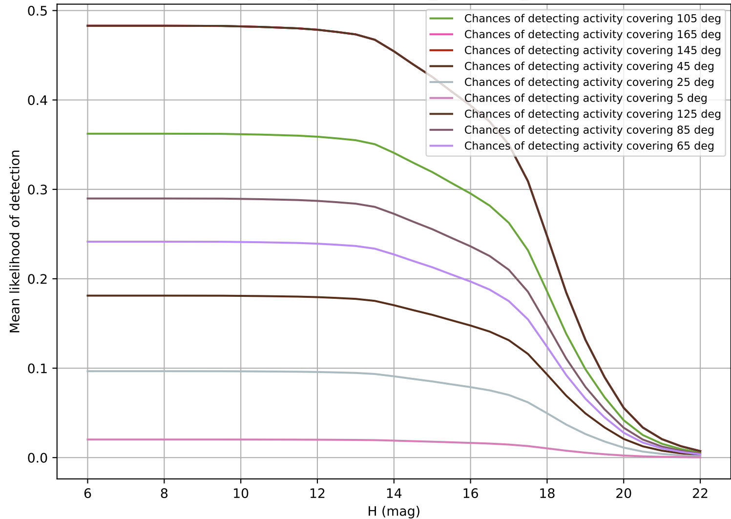
weather_cloudso16v3.4_10yrs OCC_r5
