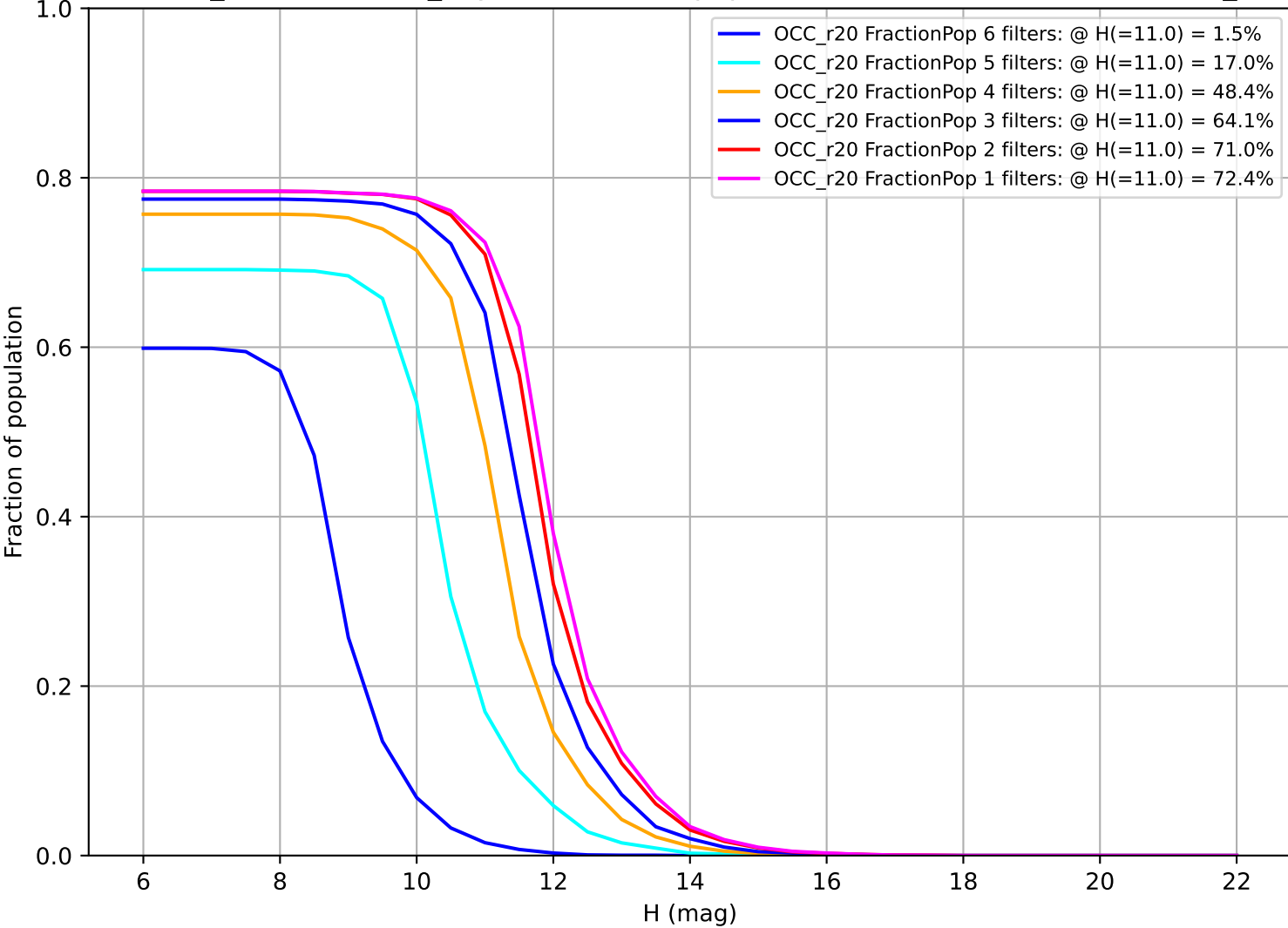
weather_cloudso16v3.4_10yrs: Fraction of population with colors in X filters OCC_r20
