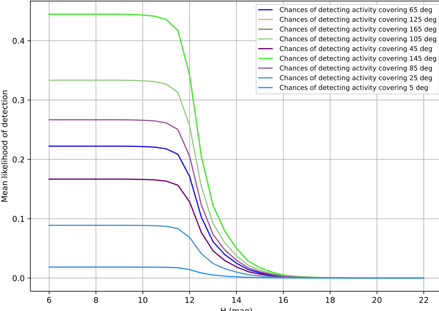
weather_cloudso16v3.4_10yrs OCC_r20
