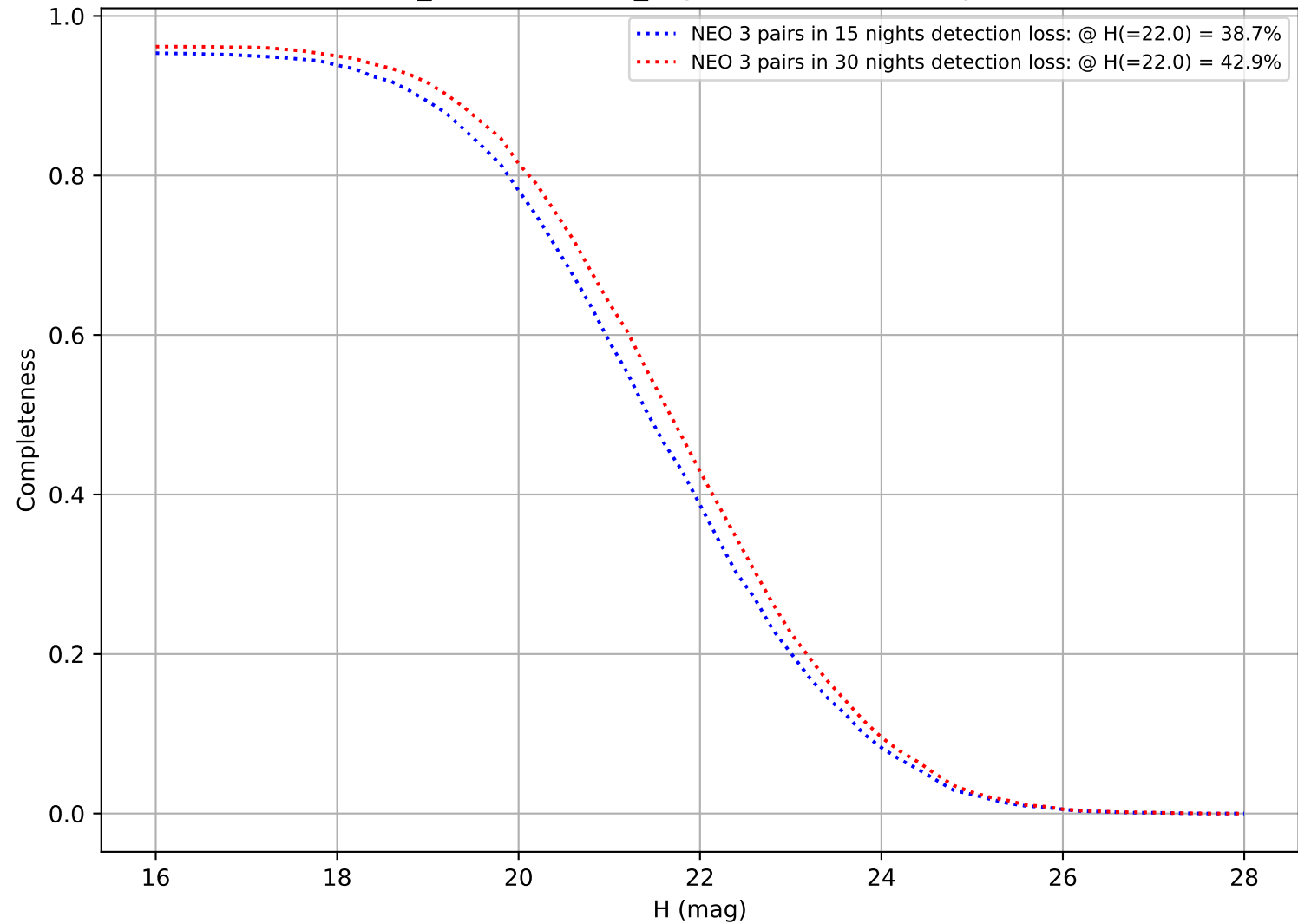
weather_cloudso16v3.4_10yrs: DifferentialCompleteness
