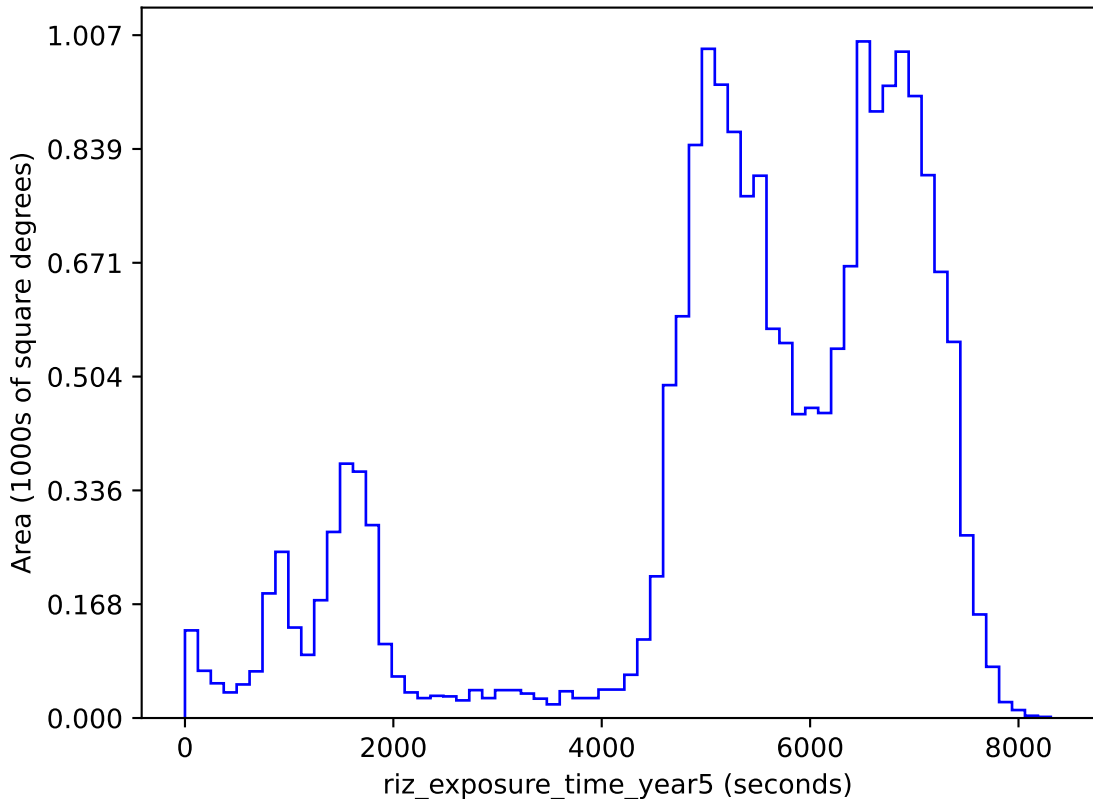
weather_cloudso16v3.4_10yrs gri band non-DD: riz_exposure_time_year5
