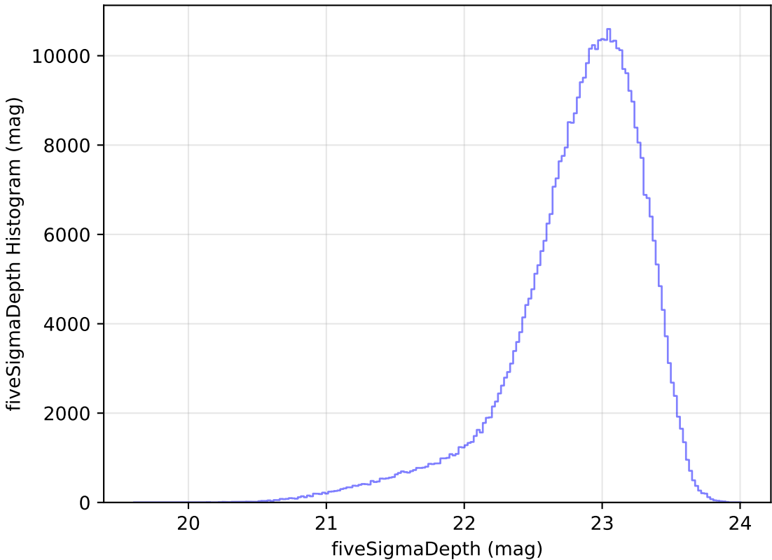
weather_cloudso16v3.4_10yrs z: fiveSigmaDepth Histogram
