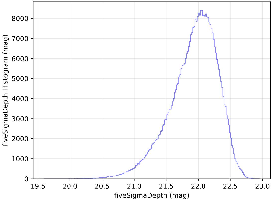
weather_cloudso16v3.4_10yrs y: fiveSigmaDepth Histogram
