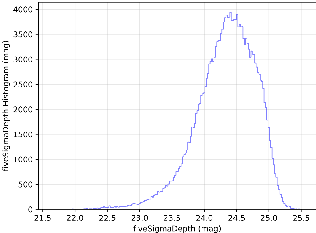
weather_cloudso16v3.4_10yrs g: fiveSigmaDepth Histogram
