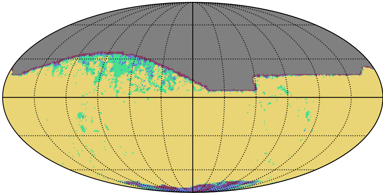
weather_cloudso16v3.4_10yrs z band: YearCoverage night
