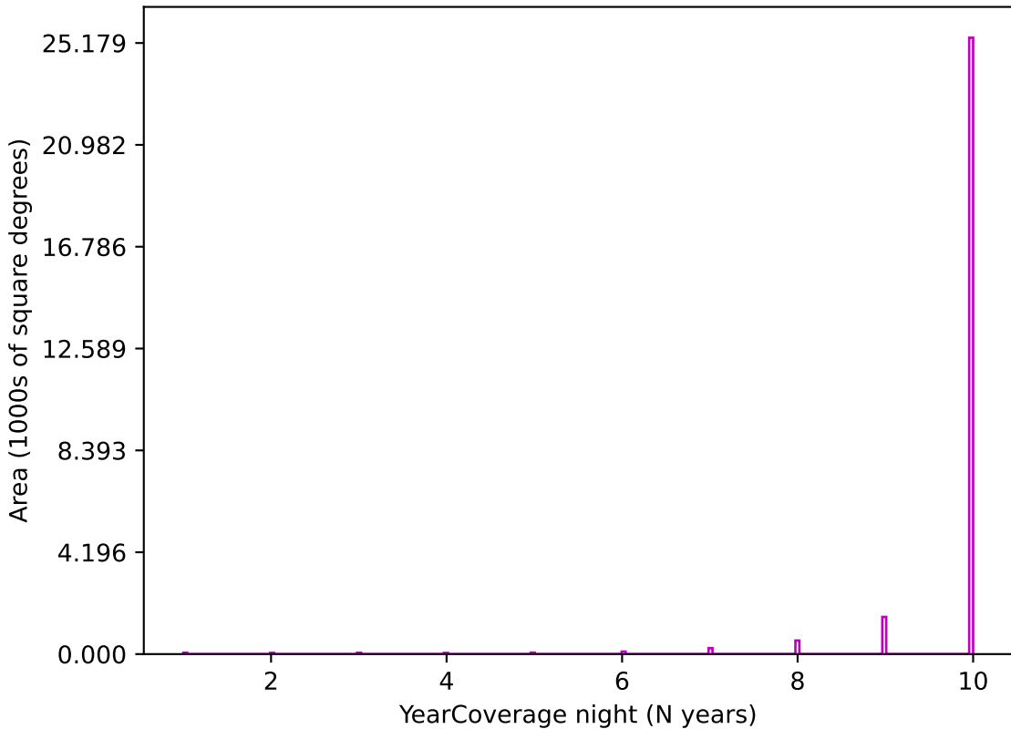
weather_cloudso16v3.4_10yrs z band: YearCoverage night
