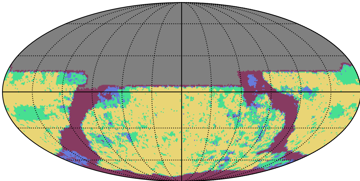
weather_cloudso16v3.4_10yrs u band: YearCoverage night
