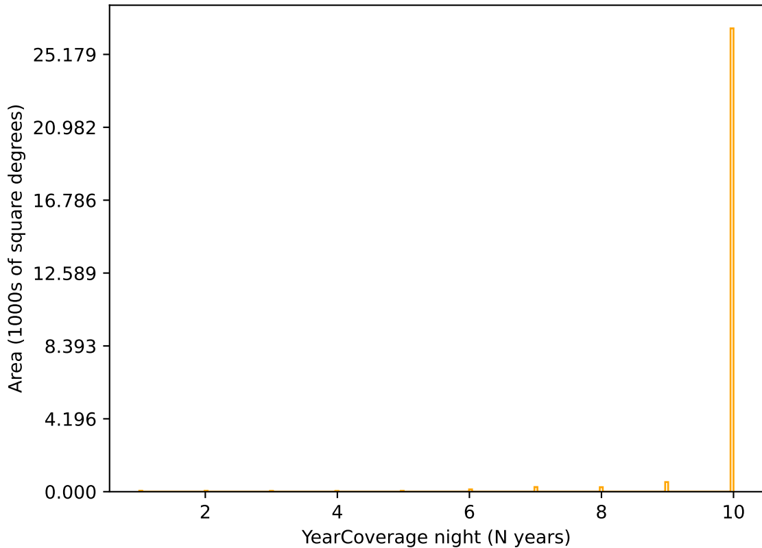
weather_cloudso16v3.4_10yrs r band: YearCoverage night
