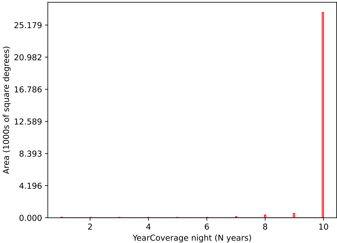
weather_cloudso16v3.4_10yrs i band: YearCoverage night
