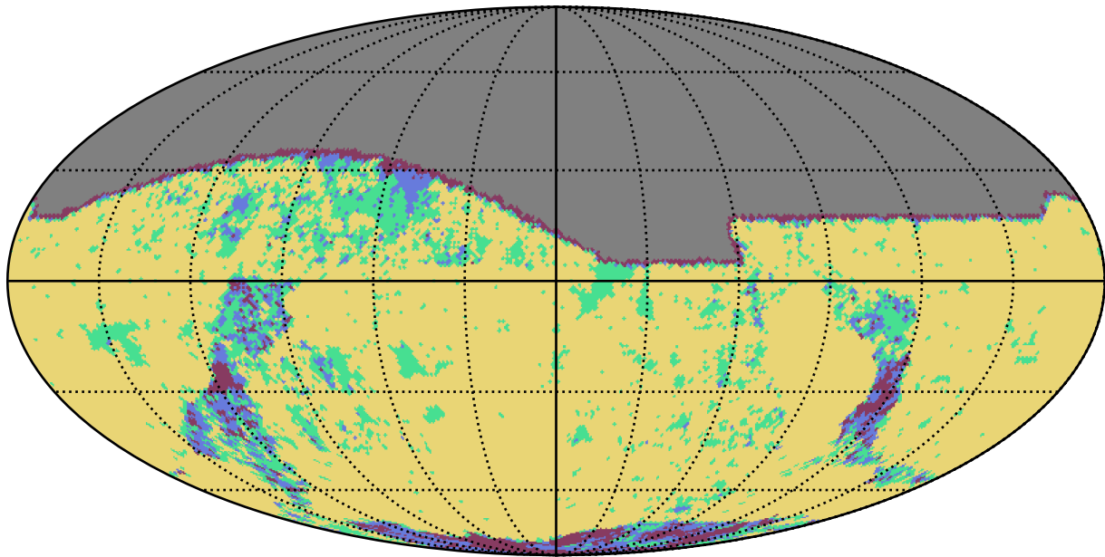
weather_cloudso16v3.4_10yrs g band: YearCoverage night
