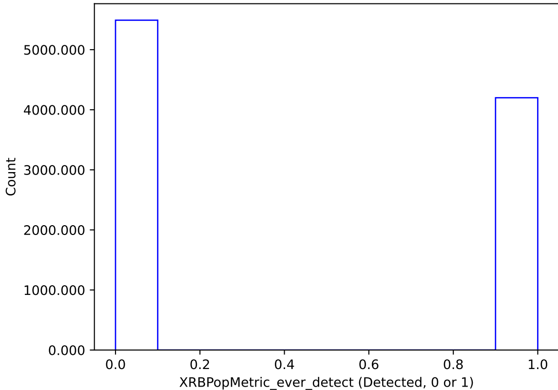
weather_cloudso16v3.4_10yrs : XRBPoMetric_ever_detect
