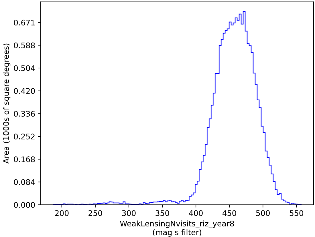
weather_cloudso16v3.4_10yrs gri band non-DD: WeakLensingNvisits_riz_year8
