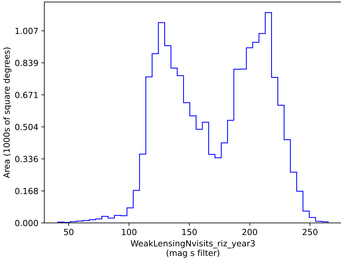
weather_cloudso16v3.4_10yrs gri band non-DD: WeakLensingNvisits_riz_year3
